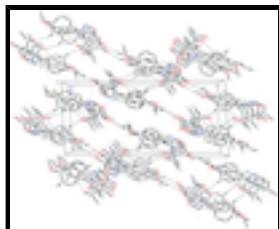
Fig. 2. The crystal packing of the title compound, viewed along the a axis. H atoms not involved in the intermolecular interactions (dashed lines) are omitted for clarity.
